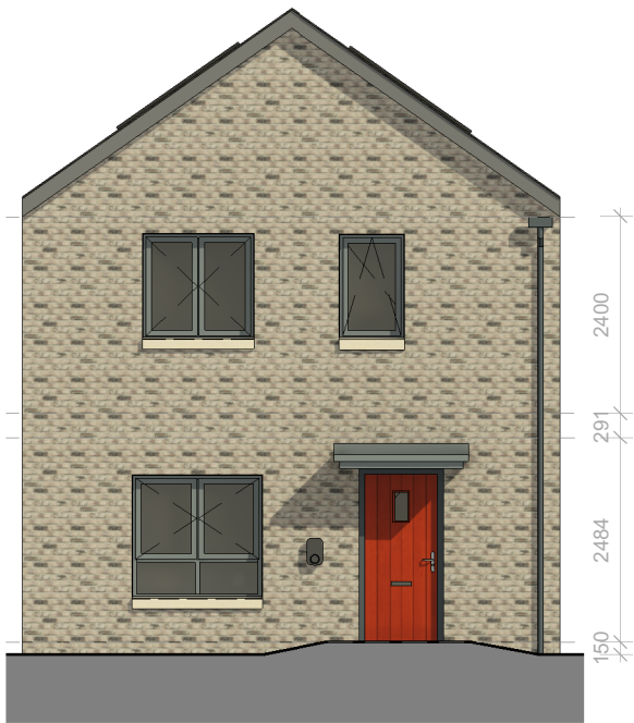
Front Elevation 1 : 100
